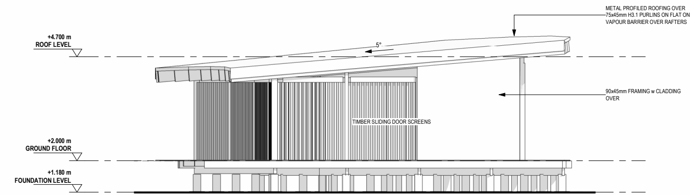
3 SIDE ELEVATION (TYP.) SCALE: 1 : 50
