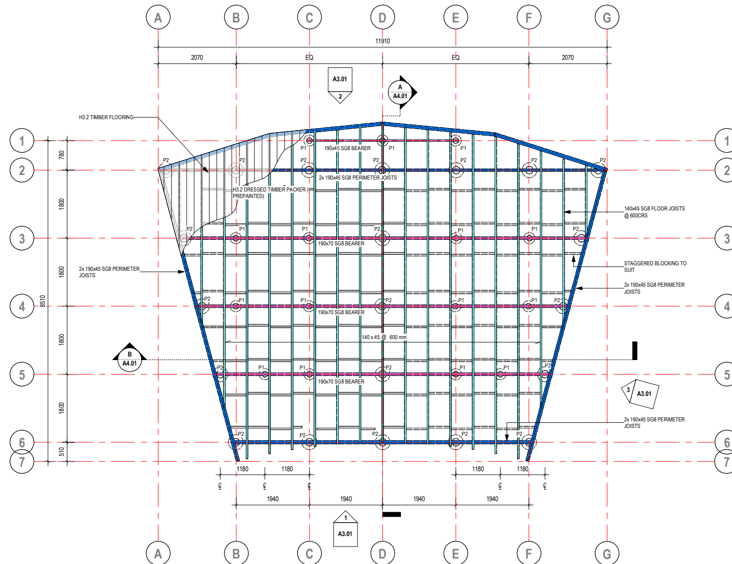
1 SUB-FLOOR/ FOUNDATION PLAN (TYP.) A3.01 SCALE: 1 : 50
