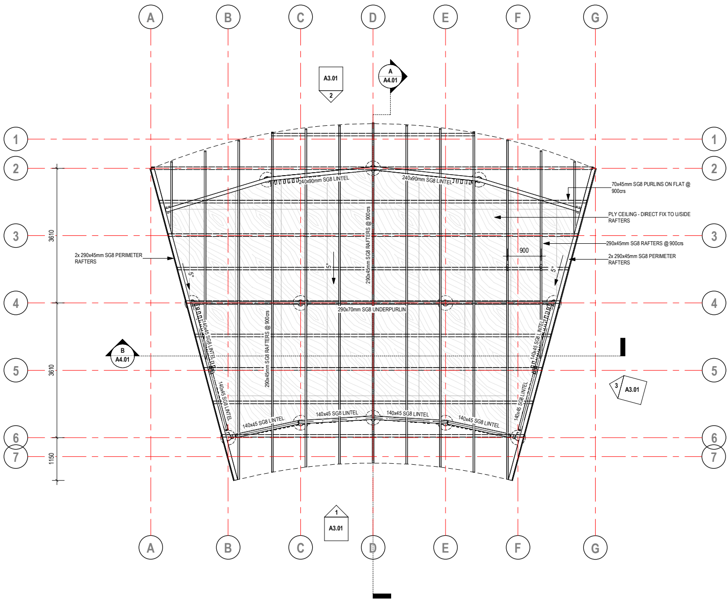
1 ROOF FRAMING PLAN A3.01 SCALE: 1 : 50
